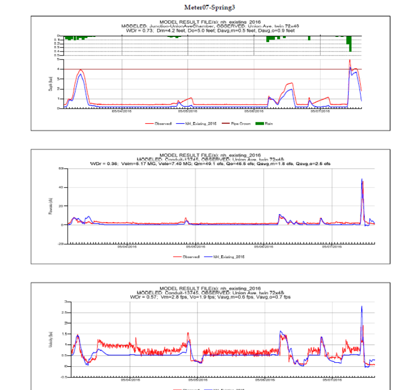
Comparison of observed and modeled data from SWMM
